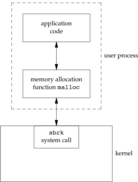
Figure 1.11 Separation of malloc function and sbrk system call
