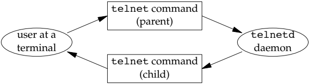
Figure 14.14 The telnet program using two processes
