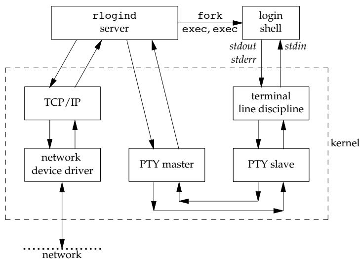
Figure 19.3 Arrangement of processes for rlogind server
