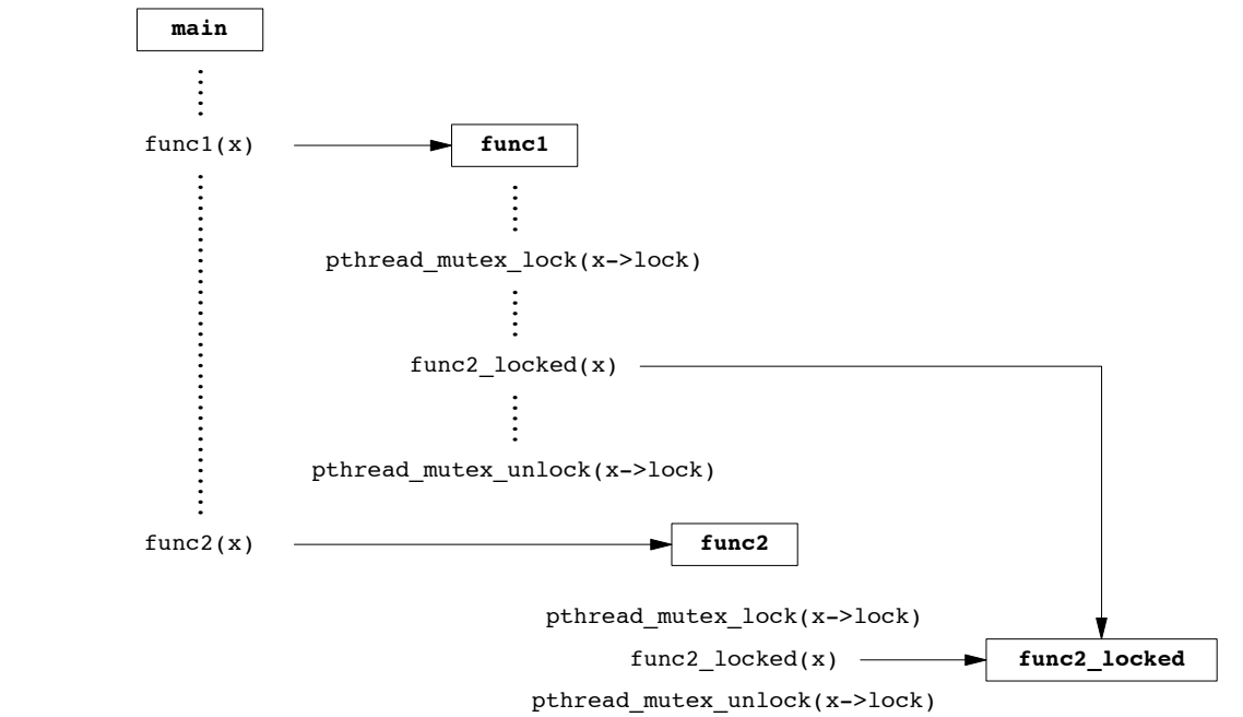
Figure 12.7 Avoiding a recursive locking opportunity
