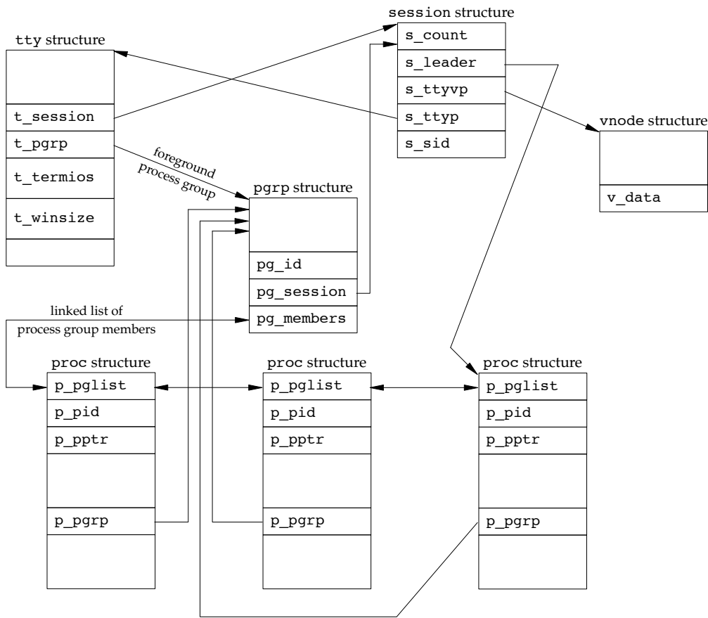
Figure 9.13 FreeBSD implementation of sessions and process groups
