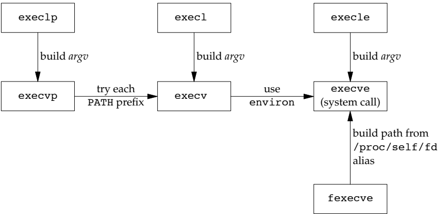
Figure 8.15 Relationship of the seven exec functions
