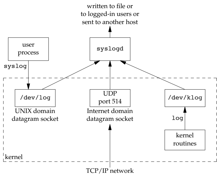
Figure 13.2 The BSD syslog facility
